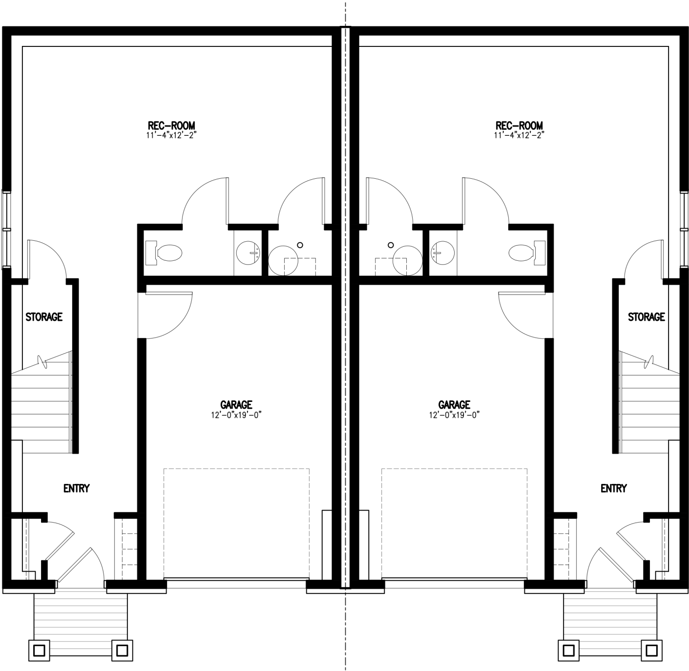
BASEMENT FLOOR
